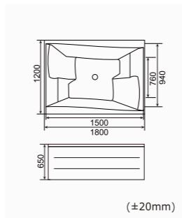
RL-6158 SKU:0350015 1800*1200*650mm(70"x47"x25") Loading Quantity:40'HQ(42pcs)
