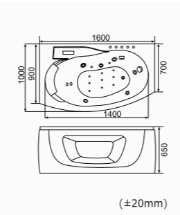
RL-6179 SKU:0350004 1600*1000*650mm(63"x39"x25") Loading Quantity:40'HQ(52pcs)
