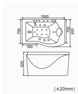
RL-6157 L/R SKU:0350024 (L)/0350025 (R) 1400*820*620mm(55"x32"x24") 1500*820*620mm(59"x32"x24") Loading Quantity:40'HQ(52pcs/50pcs)
