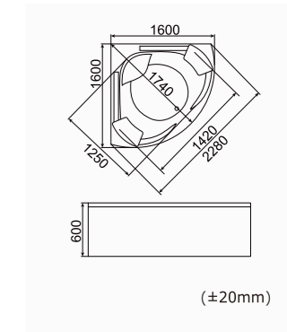
RL-6200 SKU:0350029 1600*1600*600mm(63"x63"x23") Loading Quantity:40'HQ(44pcs)
