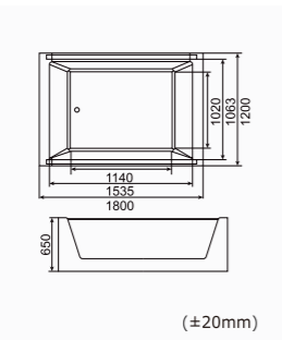
RL-6181 SKU:0350007 1800*1200*650mm(70"x47"x25") Loading Quantity:40'HQ(41pcs)
