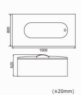
RL-H1580 SKU:0350058 1500*800*620mm(59"x31"x24") Loading Quantity:40'HQ(50pcs)
