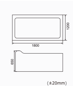
RL-H1812-1 L SKU:0350057 1800*1200*650mm(70"x47"x25") Loading Quantity:40'HQ(36pcs)
