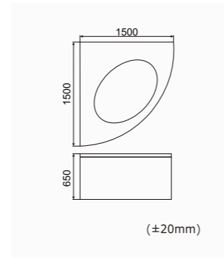
RL-H150-1 SKU:0350054 1500*1500*650mm(59"x59"x25") Loading Quantity:40'HQ(36pcs)
