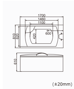
RL-6156 SKU:0350013 1700*810*610mm(67"x32"x24") Loading Quantity:40'HQ(50pcs)
