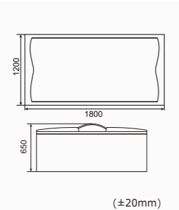
RL-H1812 L SKU:0350056 1800*1200*650mm(70"x47"x25") Loading Quantity:40'HQ(36pcs)
