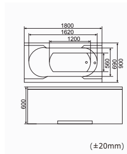
RL-6162 SKU:0350016 1800*900*600mm(70"x35"x23") Loading Quantity:40'HQ(48pcs)
