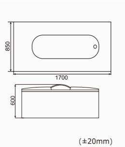
RL-H1785 SKU:0350059 1700*850*600mm(67"x33"x23") Loading Quantity:40'HQ(48pcs)
