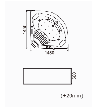
RL-6138 SKU:0350046 1450*1450*560mm(57"x57"x22") Loading Quantity:40'HQ(29pcs)
