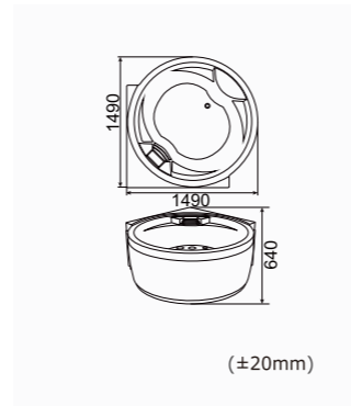
RL-6139 SKU:0350037 1490*1490*640mm(59"x59"x25") Loading Quantity:40'HQ(29pcs)
