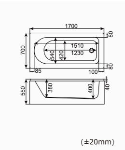
RL-6170 1700*700*550mm(55"x32"x24") Loading Quantity:40'HQ(50pcs)
