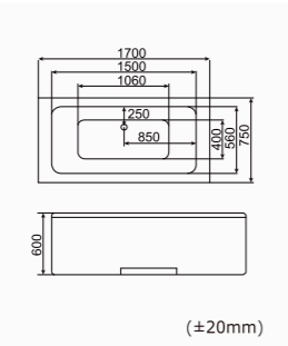
RL-6137 SKU:0350012 1700*750*600mm(67"x30"x23") Loading Quantity:40'HQ(57pcs)
