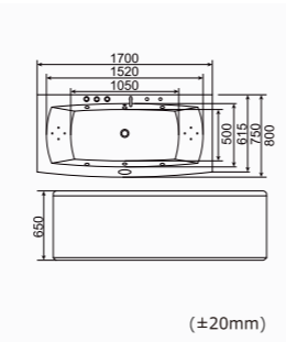
RL-6141 SKU:0350011 1700*800*650mm(67"x31"x25") Loading Quantity:40'HQ(52pcs)
