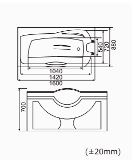
RL-6144 SKU:0350003 1600*880*700mm(63"x34"x27") Loading Quantity:40'HQ(50pcs)
